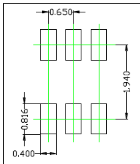
SOLDING PATTERN
