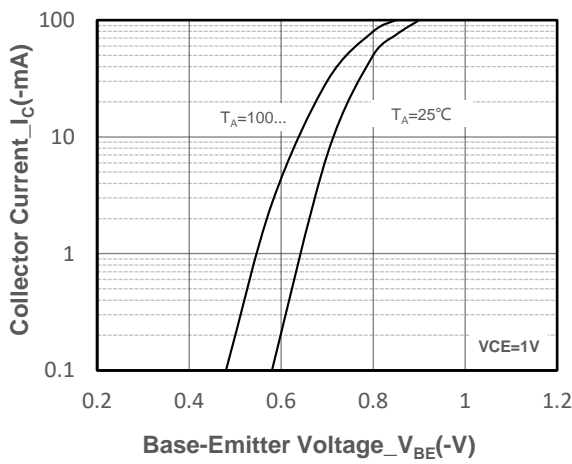
Collector Current vs. Base-Emitter Voltage
